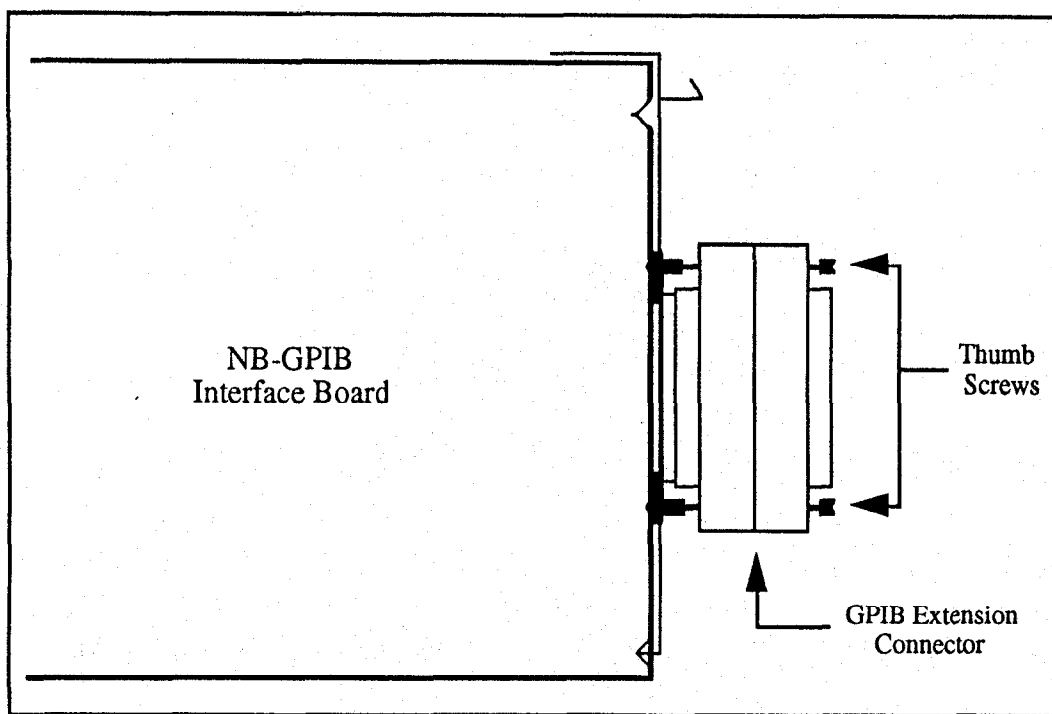
Figure 2-3. The GPIB Extension Connector
