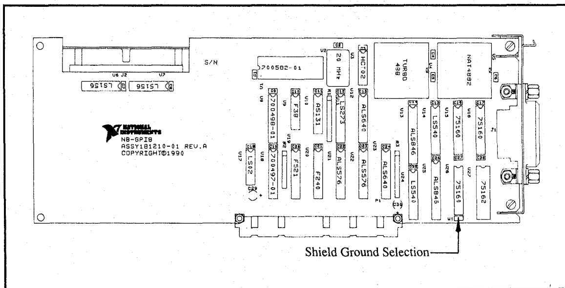
Figure 2-1. NB-GPIB Parts Locator Diagram
